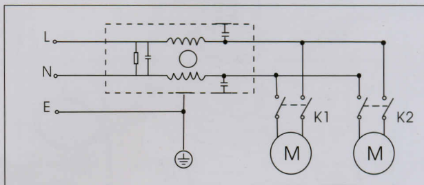
Circuit diagram
